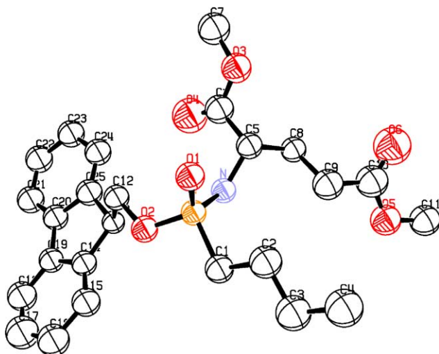
Figure 2. X-ray crystal structure of phosphonamidate 11a .
